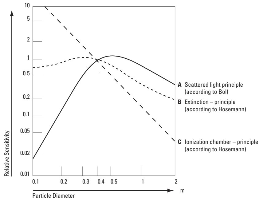
Figure 1: Relative Sensivities of Three Technologies as a Function of Particle Diameter (Source: NBS IR78-1502, “Smoke Measurements In Large and Small Scale Fire Testing,” by Richard W. Bukowski)
