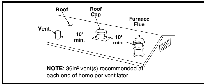
Figure 5. Roof Spacing
