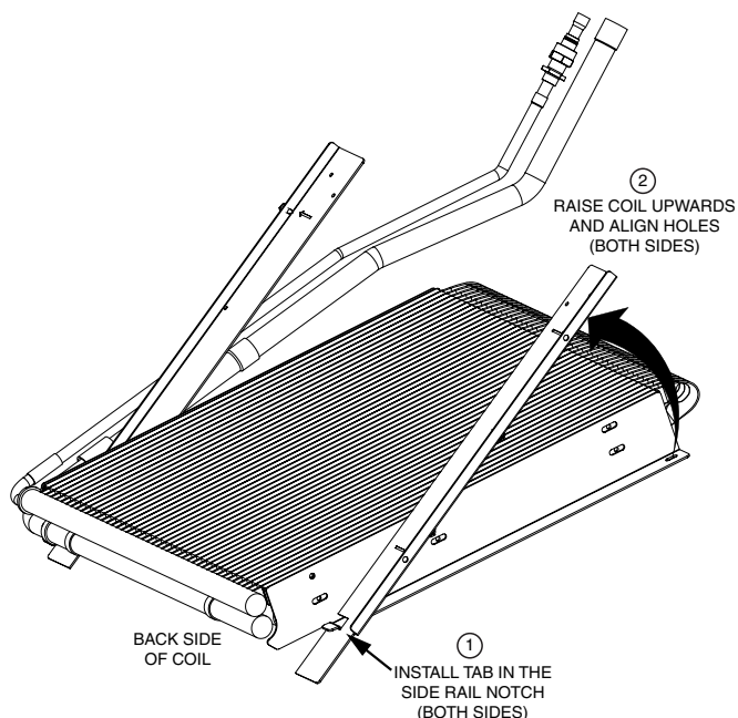
Figure 2. Coil Installation
