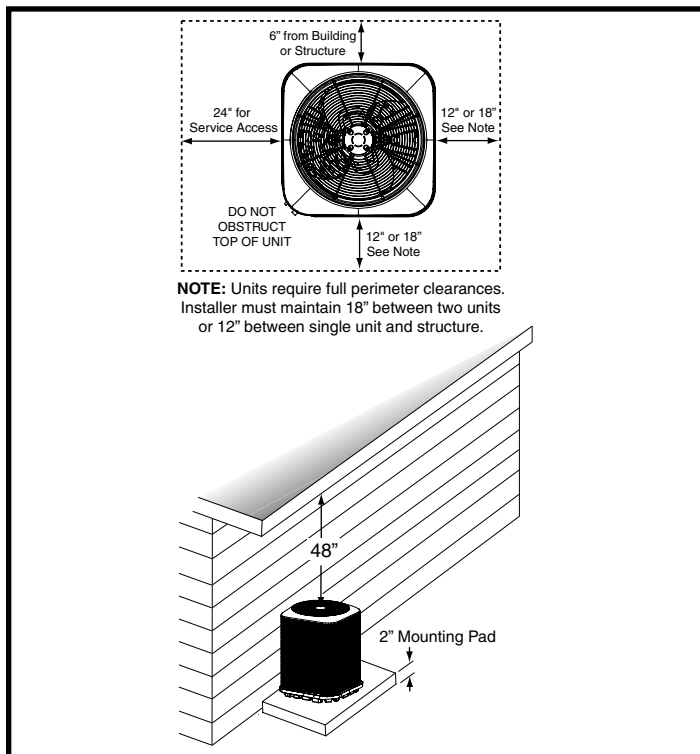
Figure 1. Clearance Requirements
